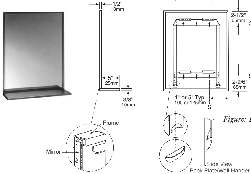
(Rear View)
